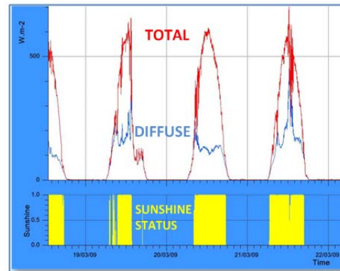
Figure 2 Graphical representation of the SPN1 readings logged over several days.
